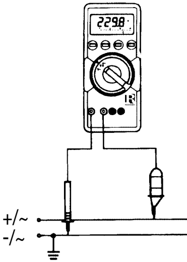
Voltage measurement on electrical systems up to 1000 V with the KS30 measuring adapter
