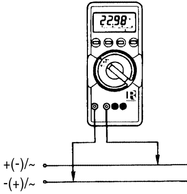
Voltage measurement
